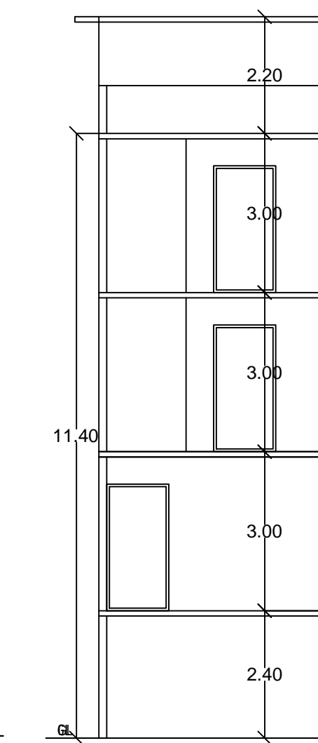
SECTION X-X
